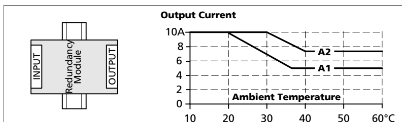
Fig. 18-8 Mounting Orientation E (Horizontal ccw)
