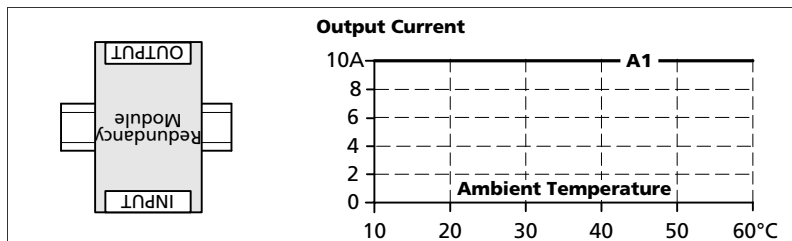
Fig. 18-5 Mounting Orientation B (Upside down)
