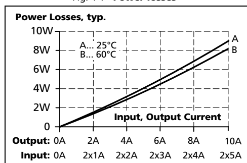
Fig. 4-1 Power losses
