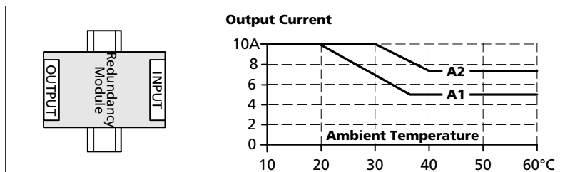
Fig. 18-7 Mounting Orientation D (Horizontal cw)
