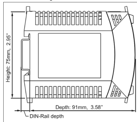
Fig. 16-2 Side view
