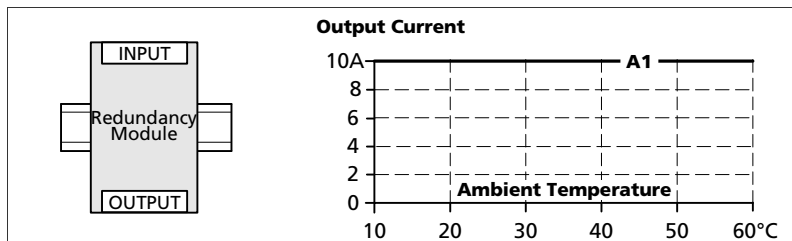
Fig. 18-4 Mounting Orientation A (Standard orientation)
