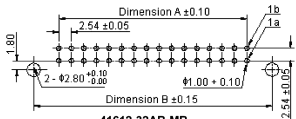
41612-32AB-MR
