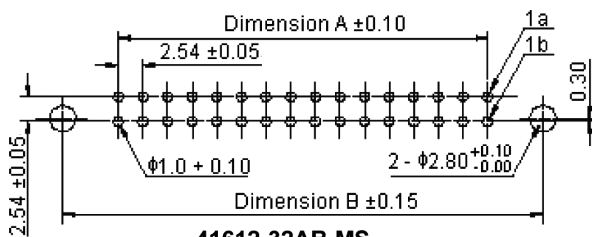
41612-32AB-MS
