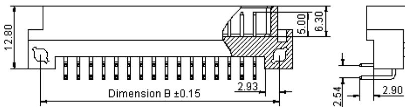
41612-32AB-MR
