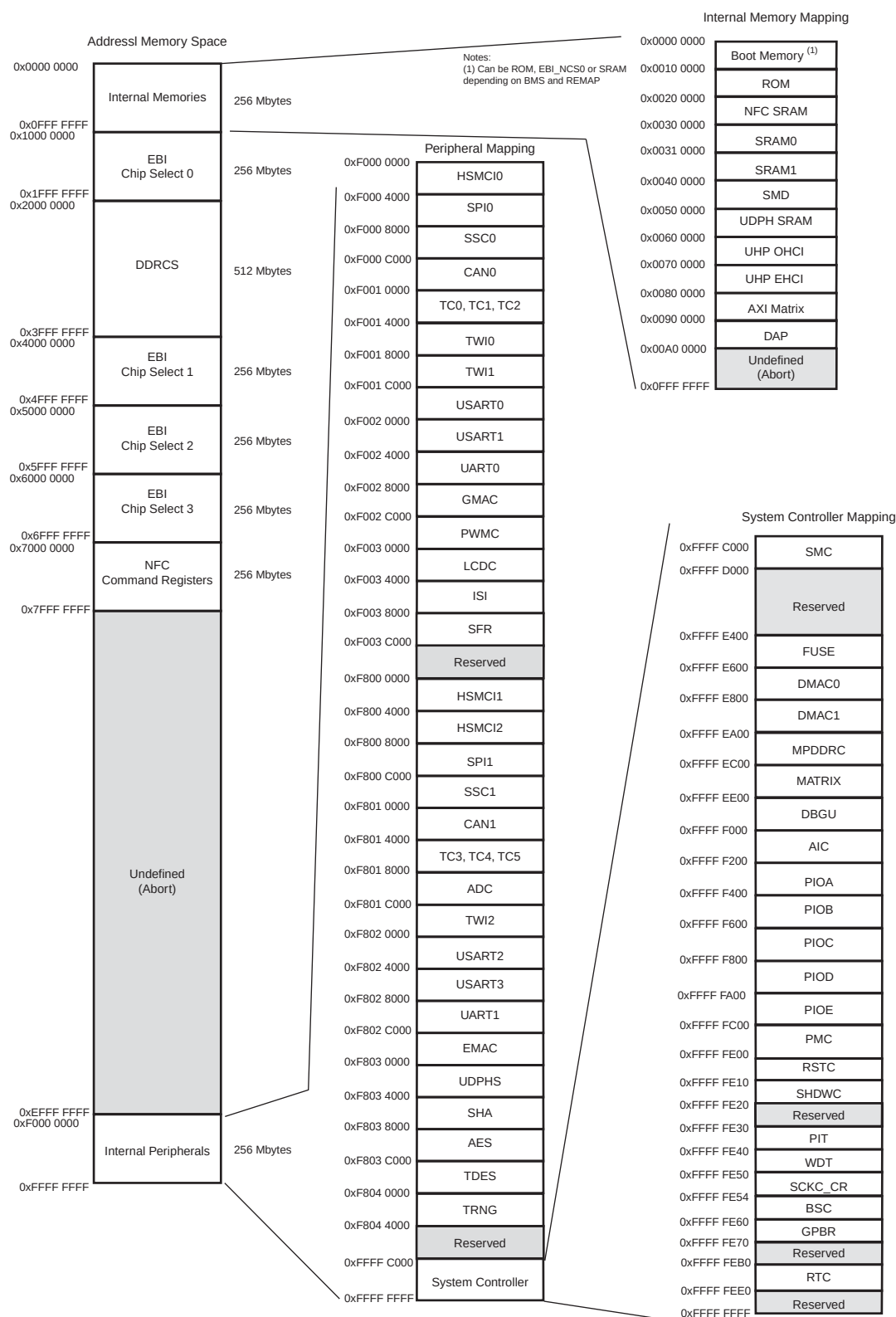
Figure 5-1. Memory Mapping
