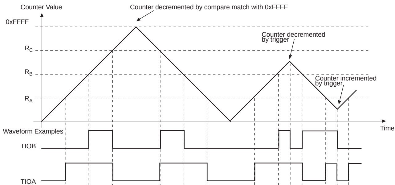
Figure 47-12. WAVSEL = 01 with Trigger
