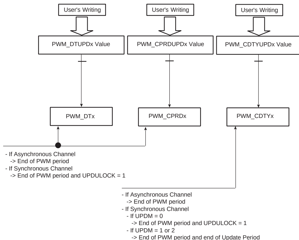
Figure 48-16. Synchronized Period, Duty-Cycle and Dead-Time Update
