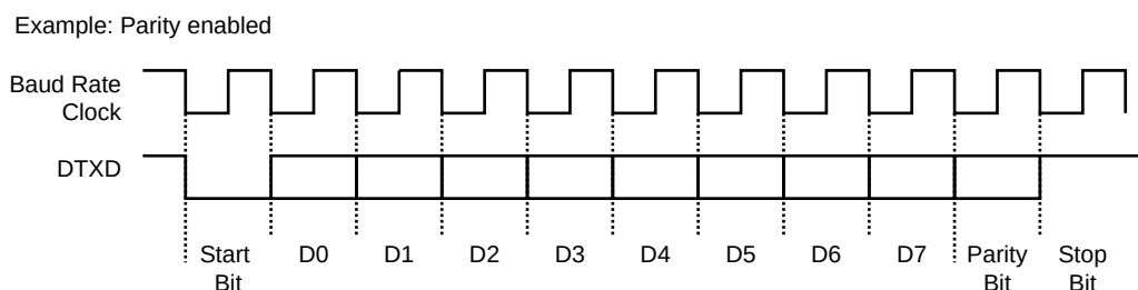
Figure 42-10. Character Transmission
