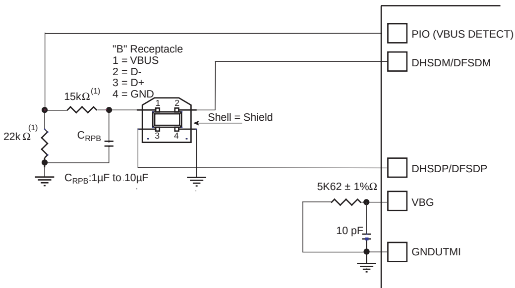
Figure 56-3. Typical USB High Speed Device Connection
