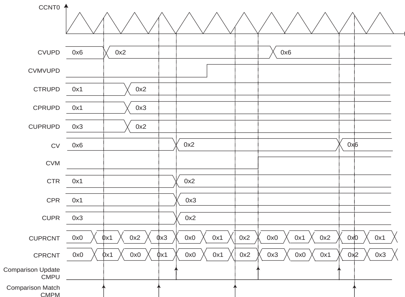
Figure 48-13. Comparison Waveform
