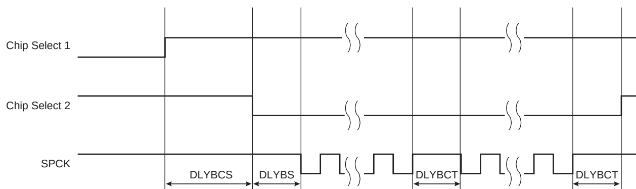
Figure 39-9. Programmable Delays
