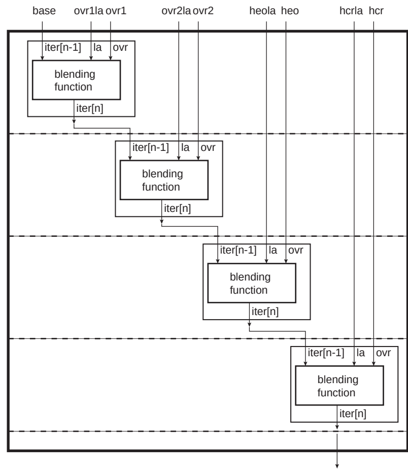
Figure 32-13. Global Alpha Blender
