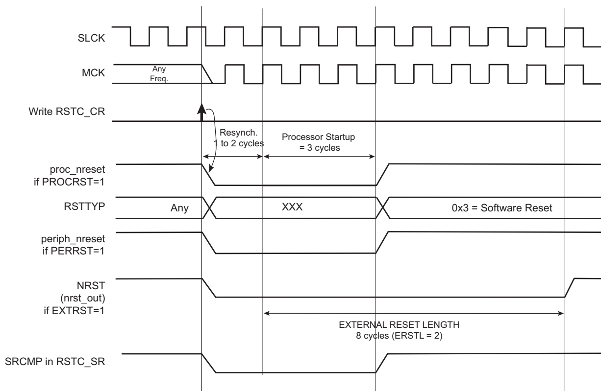
Figure 18-7. Software Reset
