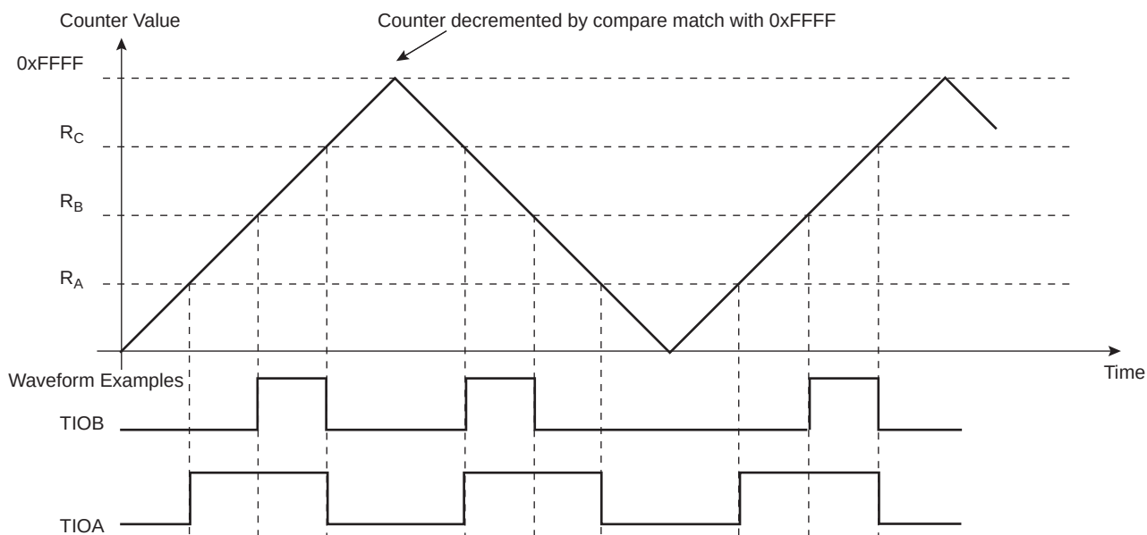
Figure 47-11. WAVSEL = 01 without Trigger
