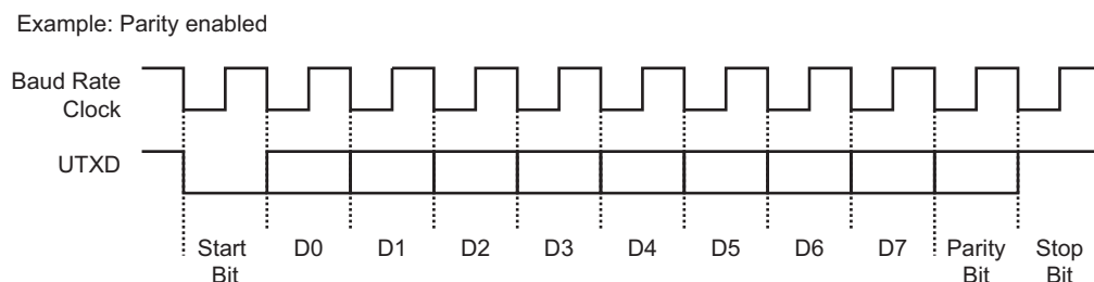
Figure 43-9. Character Transmission
