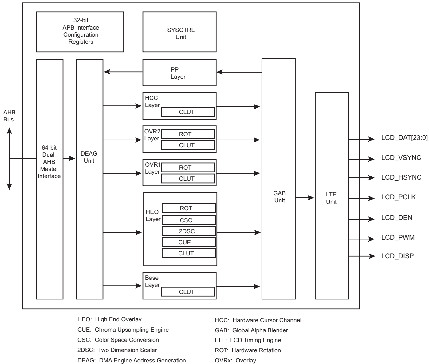
Figure 32-1. Block Diagram
