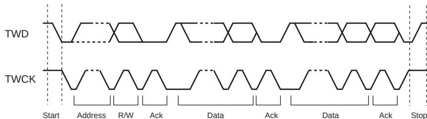
Figure 40-3. Transfer Format
