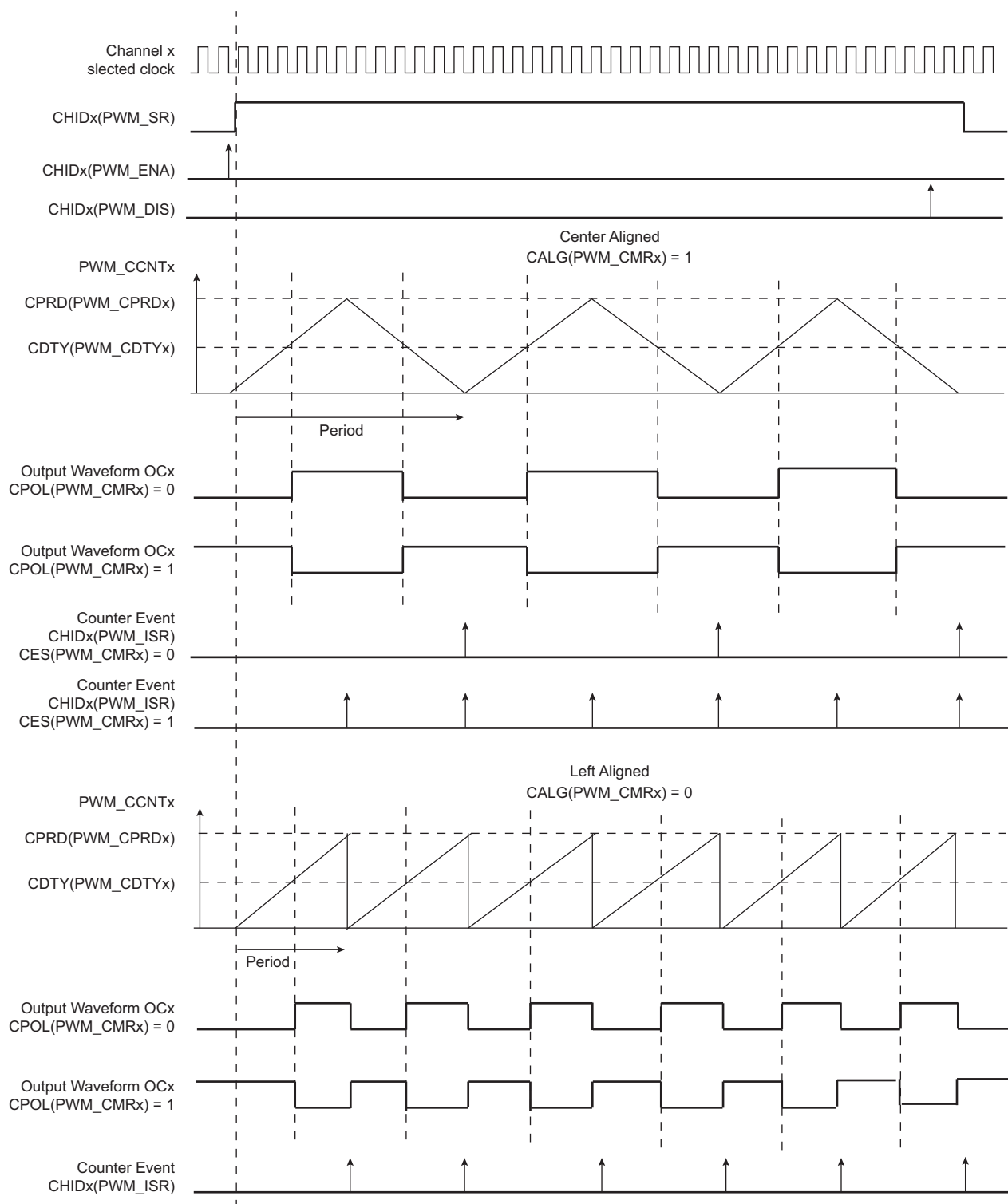
Figure 48-5. Waveform Properties
