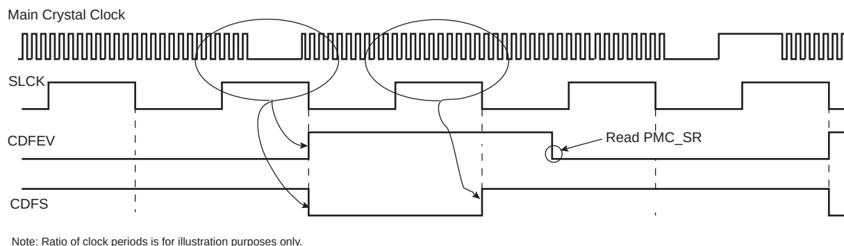
Figure 26-5. Clock Failure Detection (Example)
