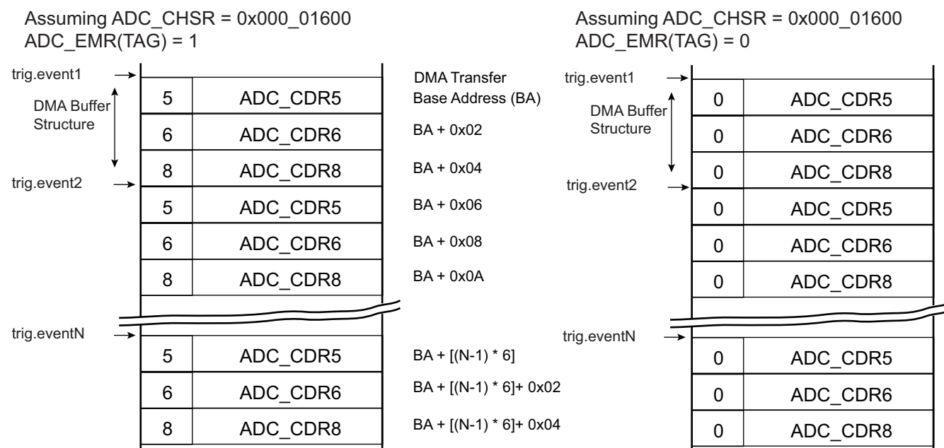
Figure 49-15. Buffer Structure
