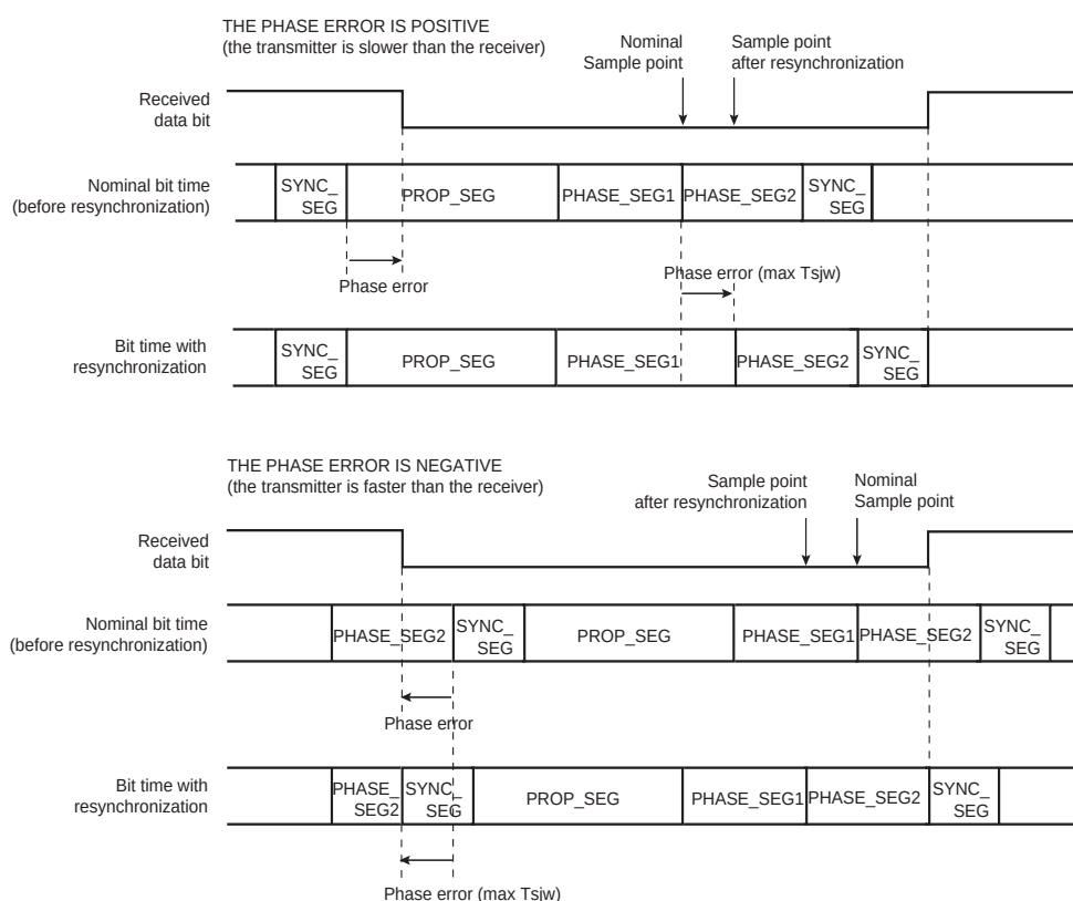
Figure 45-6. CAN Resynchronization
