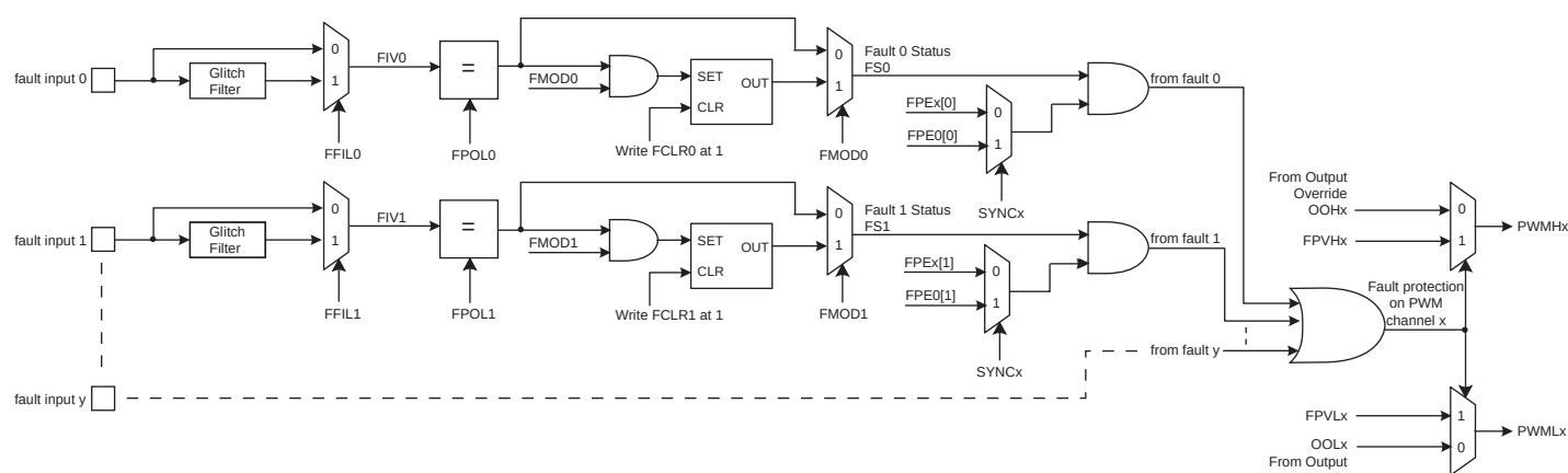
Figure 48-9. Fault Protection
