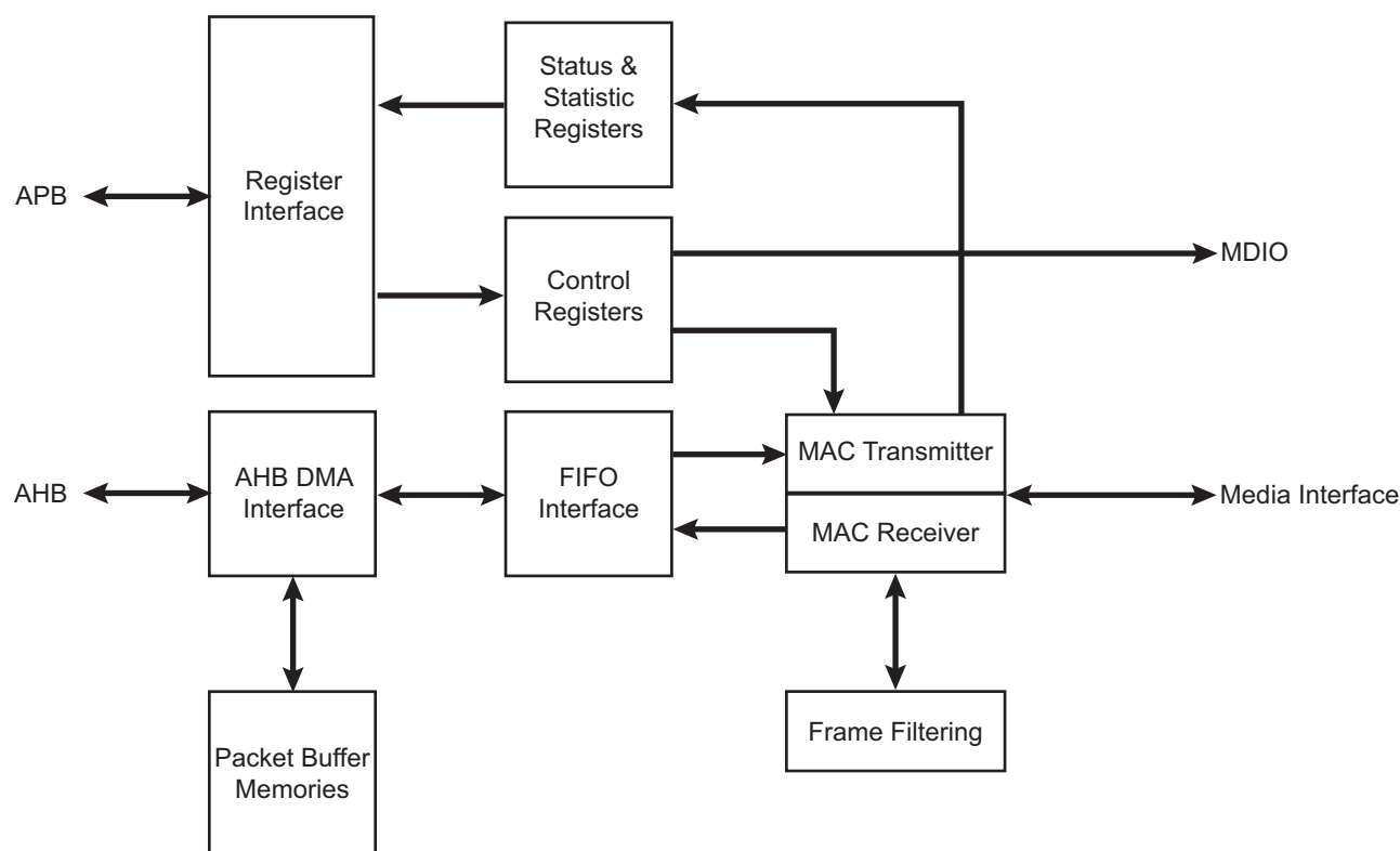
Figure 36-1. Block Diagram
