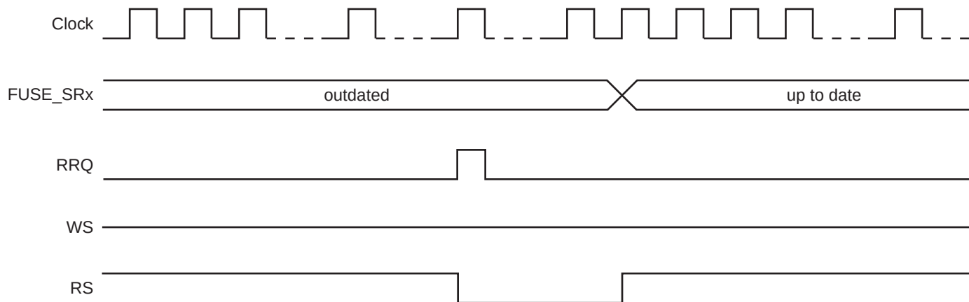
Figure 24-2. Fuse Read
