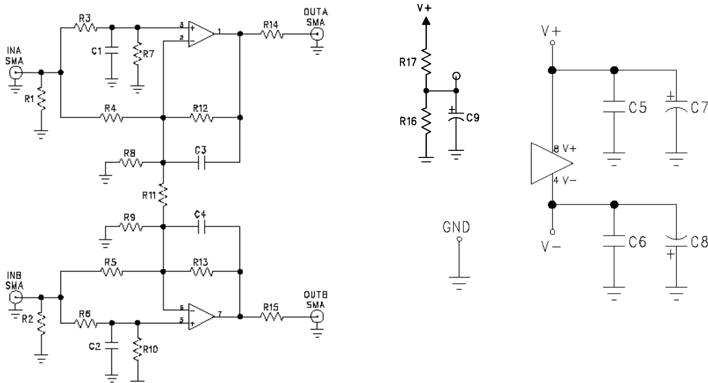
Figure 1: Complete Evaluation Board Schematic
