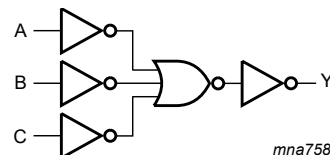
Fig. 3. Logic diagram (one gate)
