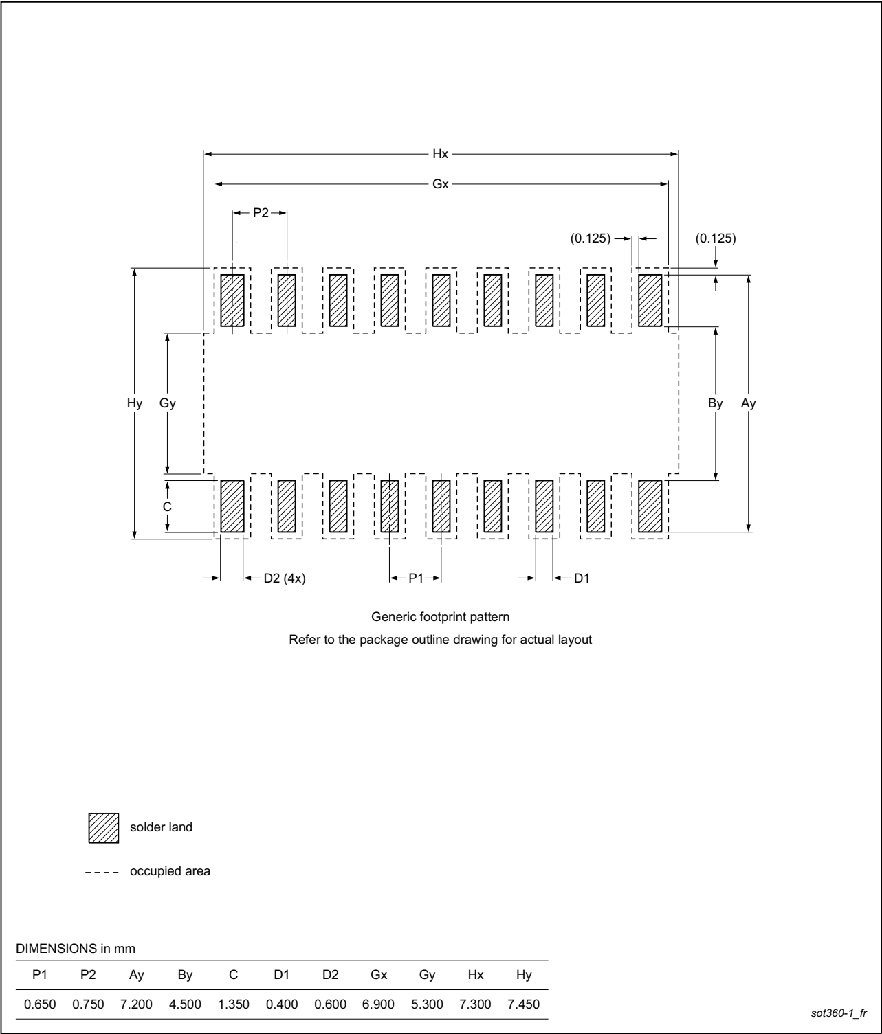
Fig 24. PCB footprint for SOT360-1 (TSSOP20); reflow soldering
