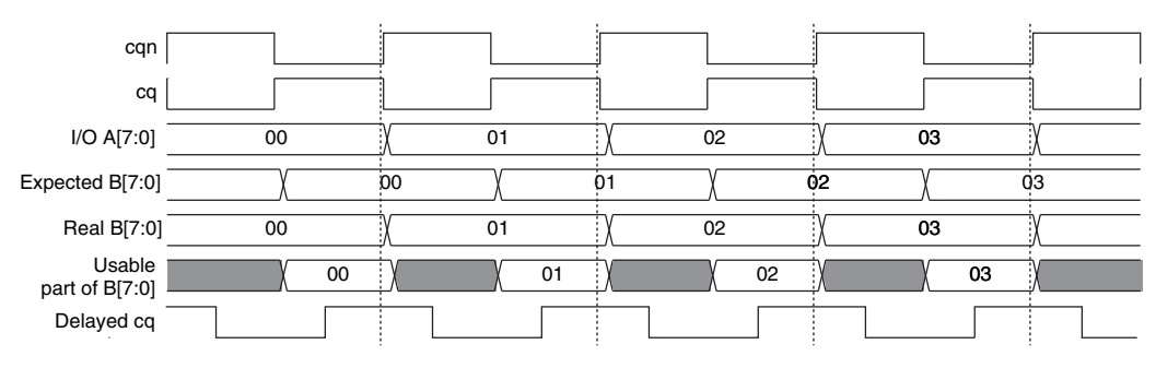
Figure 3–6. Timing Diagram of the IOE
