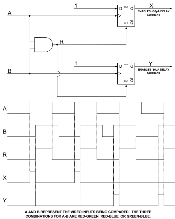
FIGURE 15. DELAY DETECTOR
