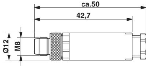
Dimensioned drawing
