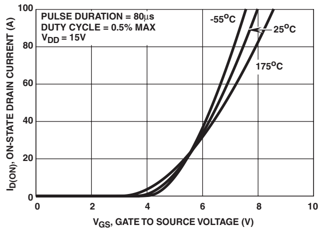
FIGURE 8. TRANSFER CHARACTERISTICS
