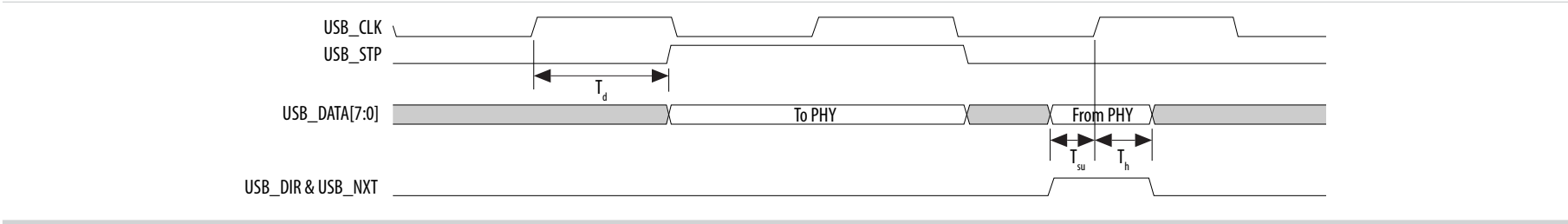
Figure 9: USB Timing Diagram
