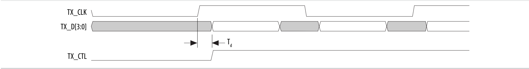
Figure 10: RGMII TX Timing Diagram
