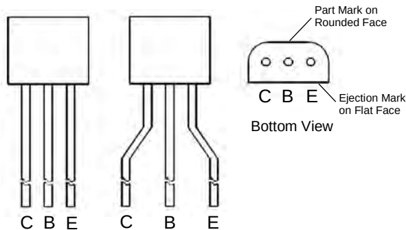
Pin-Out Configuration
