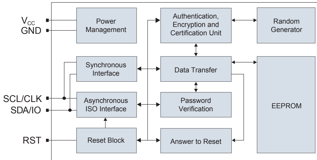
Figure 2. Block Diagram
