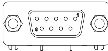
FEMALE, 9 CONTACT D-SUB CONNECTOR
