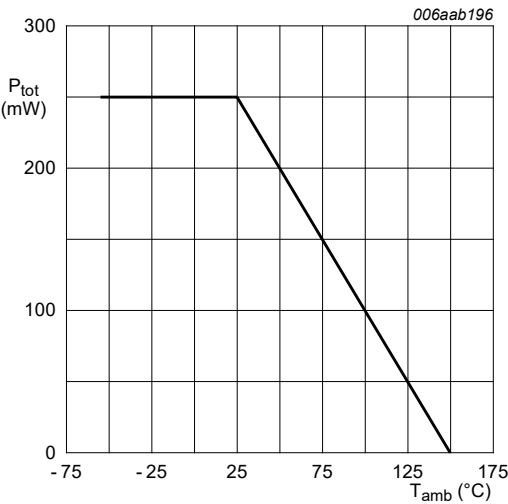
Fig. 1. Power derating curve SOT23 (TO-236AB)
