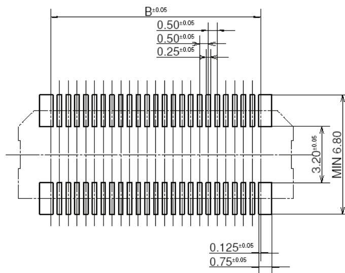
Recommended PC board pattern (TOP VIEW)
