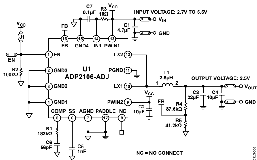
Figure 10. Evaluation Board Schematic for ADP2106-EVAL with Adjustable V_{OUT} Initially Set to 2.5 V
