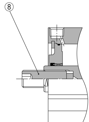
Male thread
