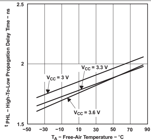
Figure 6. Driver High-to-Low Level Propagation Delay Time vs Free-Air Temperature
