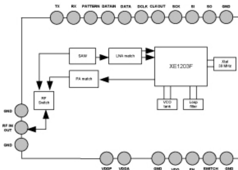
Figure 2: Antenna Switch
