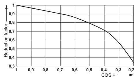
Service life reduction factor with various \text{cos } \varphi
