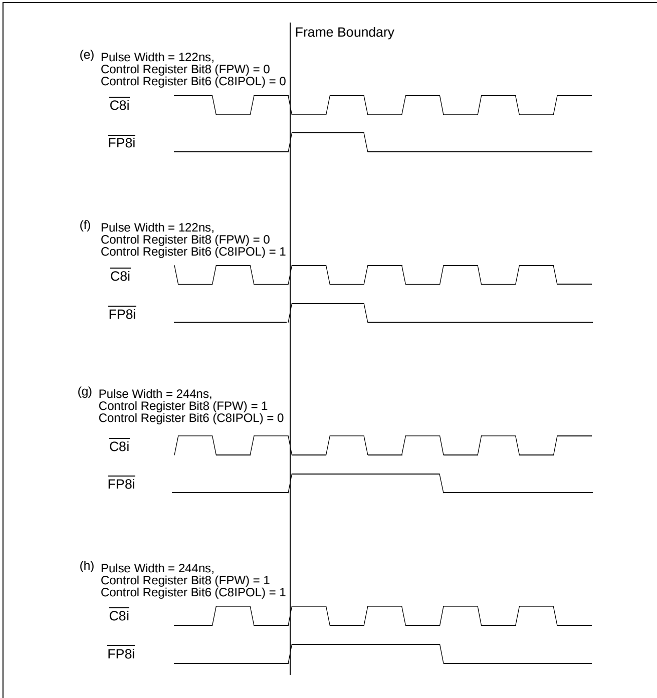
Figure 16 - Frame Boundary Conditions, GCI-Bus Operation
