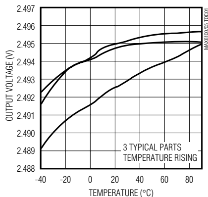
MAX6102 OUTPUT VOLTAGE TEMPERATURE DRIFT
