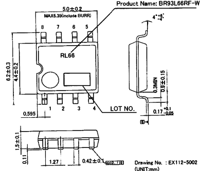
Fig4-(b) PHYSICAL DIMENSION SOP8 (BR93L46RF-W)
