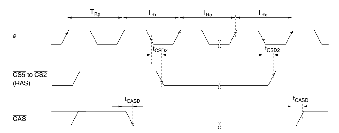
Figure 22-13 Self-Refresh Timing
