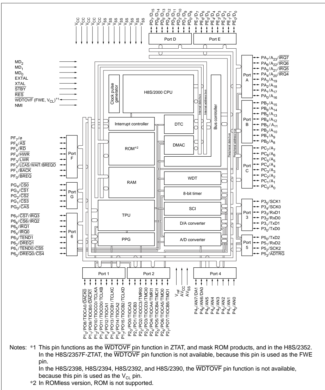
Figure 1-1 Block Diagram
