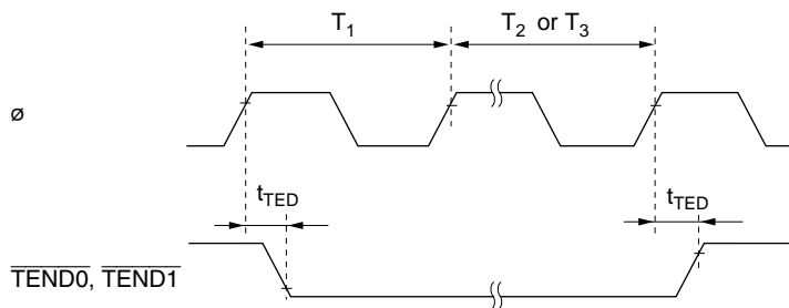
Figure 22-84 DMAC \overline{\text{TEND}} Output Timing
