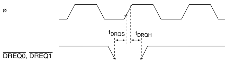
Figure 22-85 DMAC \overline{\text{DREQ}} Input Timing
