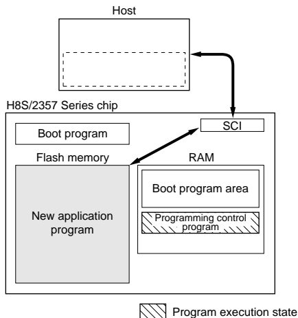
Figure 19-9 Boot Mode
