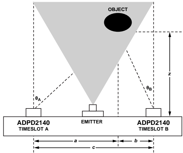
Figure 12. Triangulation Distance Measurement with the ADPD2140
