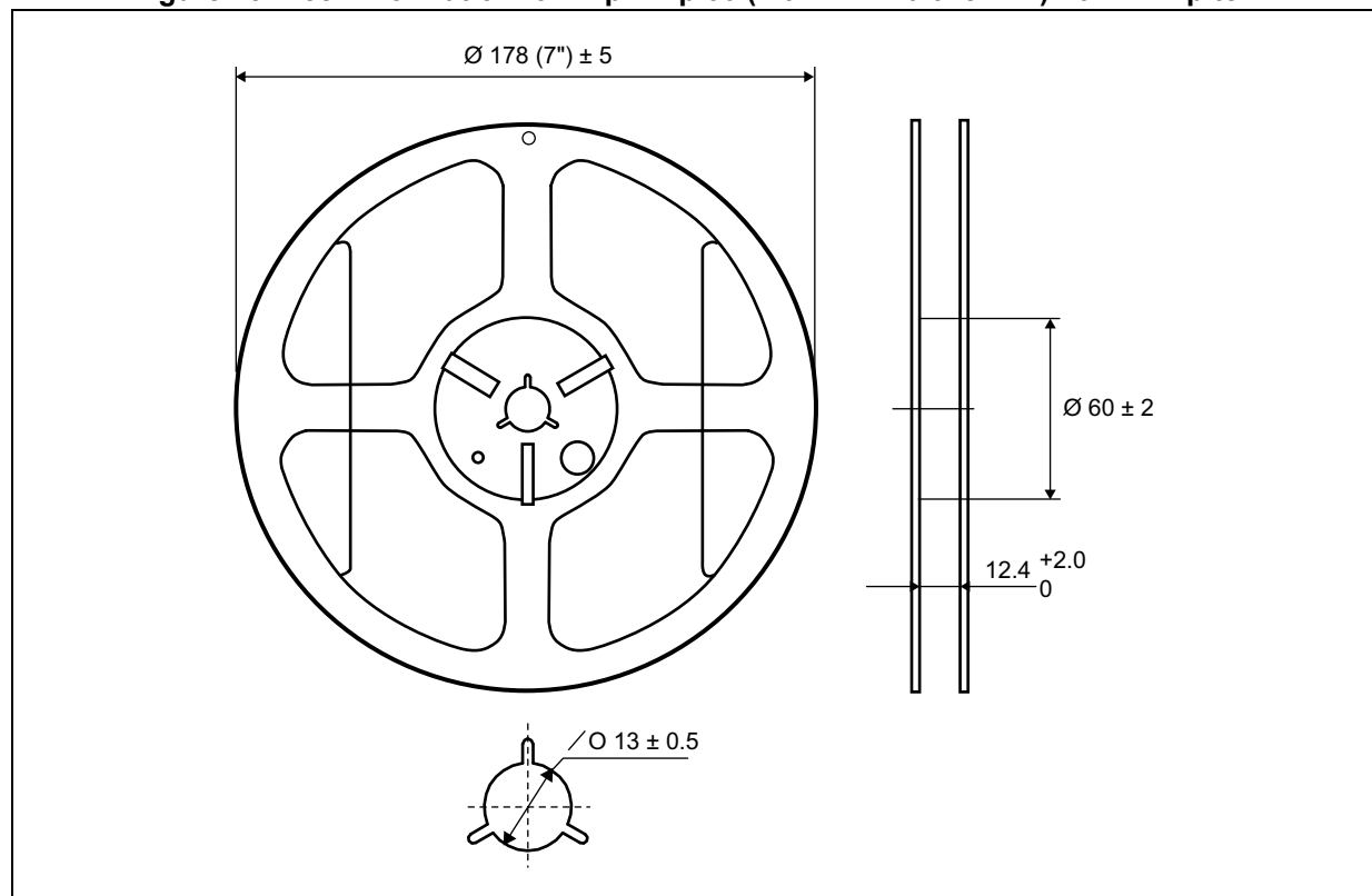
Figure 15. Reel information for Flip Chip 30 (2.0 x 2.4 x 0.625 mm) - 0.4 mm pitch
