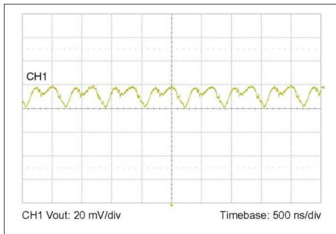
Figure 6 — Output voltage ripple at full load and 48 V F with 9.4 μF ceramic POL bypass capacitance and 20 nH distribution inductance.
