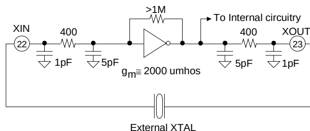
Figure 10. On-Chip Gate Oscillator Model
