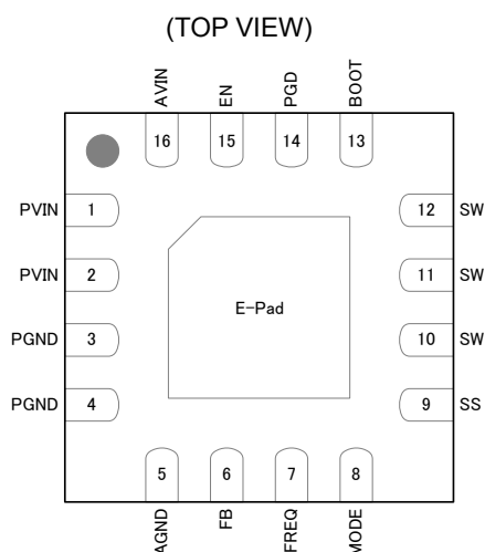
Figure 2. Pin Assignment
