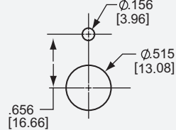
Mounting Detail Single Pole
