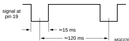
Fig.4 Output diagram of command acknowledge.
