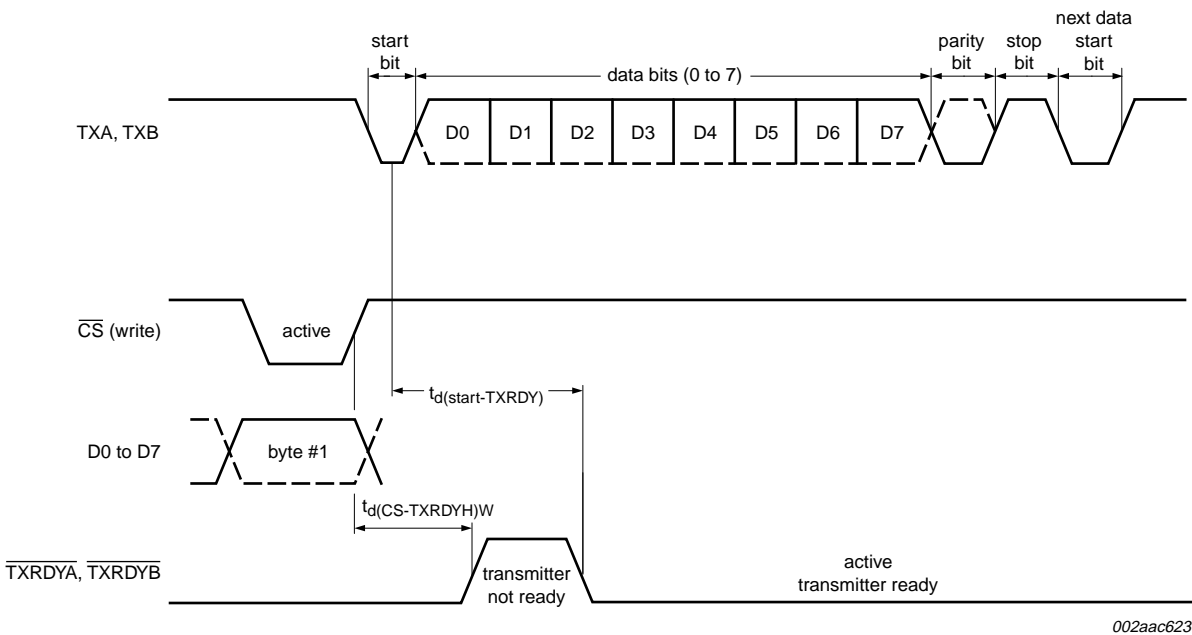
Fig 25. Transmit ready timing in non-FIFO mode (68 mode)
