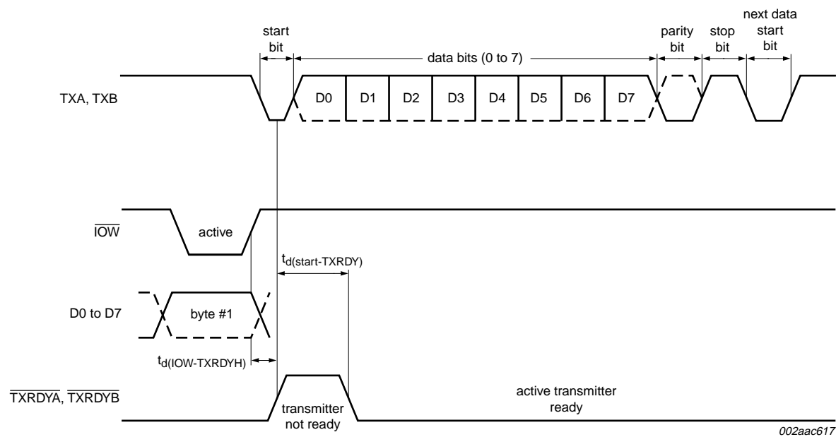
Fig 24. Transmit ready timing in non-FIFO mode (16 mode)
