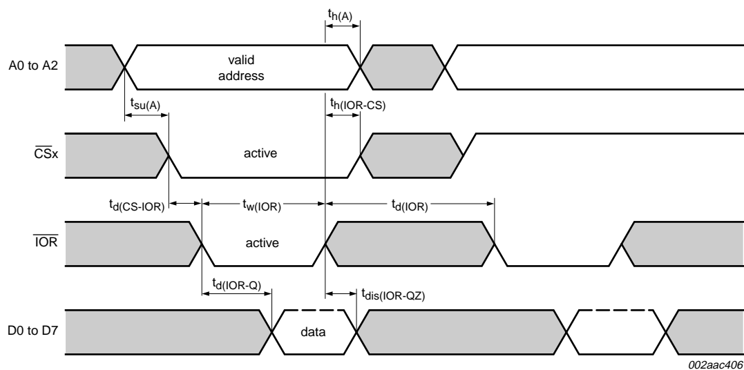
Fig 11. General read timing in 16 mode
