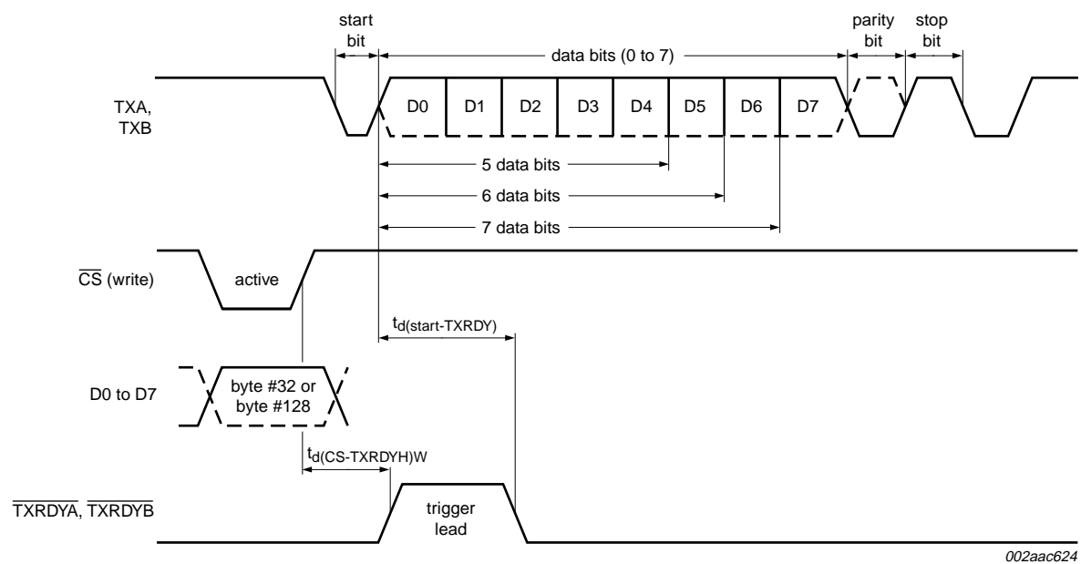
Fig 27. Transmit ready timing in FIFO mode (DMA mode '1') in 68 mode
