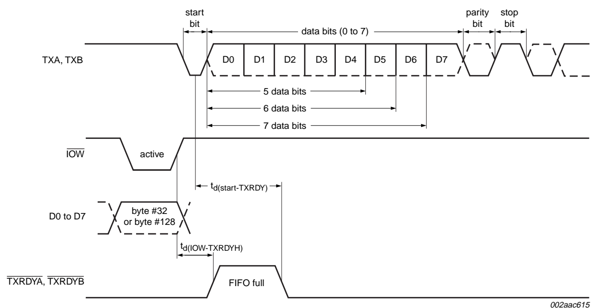
Fig 26. Transmit ready timing in FIFO mode (DMA mode '1') in 16 mode
