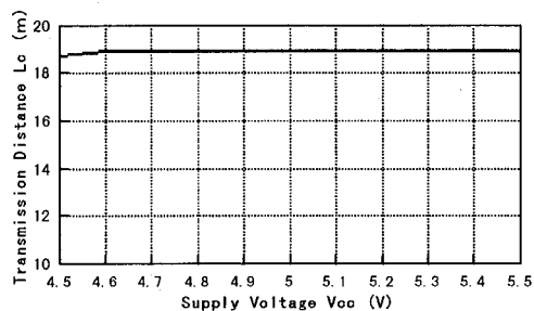
Transmission Distance vs. Supply Voltage ( T_a=25^\circ\text{C} )
