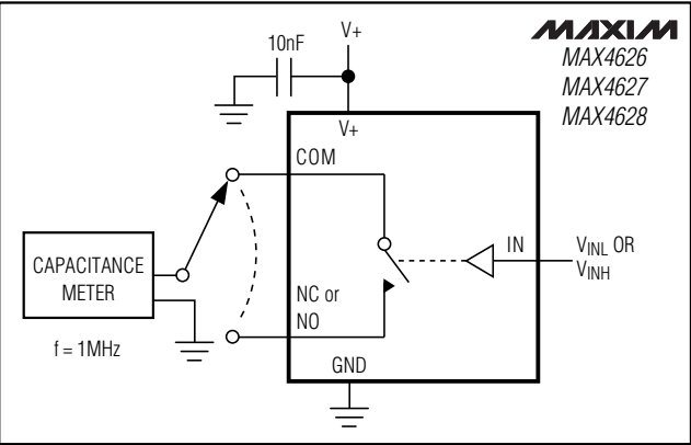
Figure 5. Channel Off/On-Capacitance
