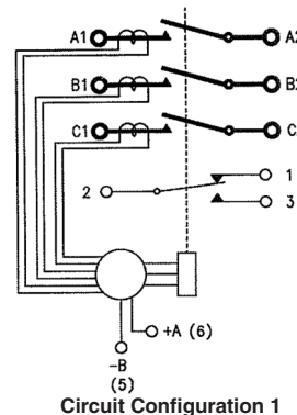
Circuit Configuration 1
