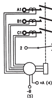
Circuit Configuration 1
