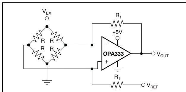
Figure 21. Single Op Amp Bridge Amplifier
