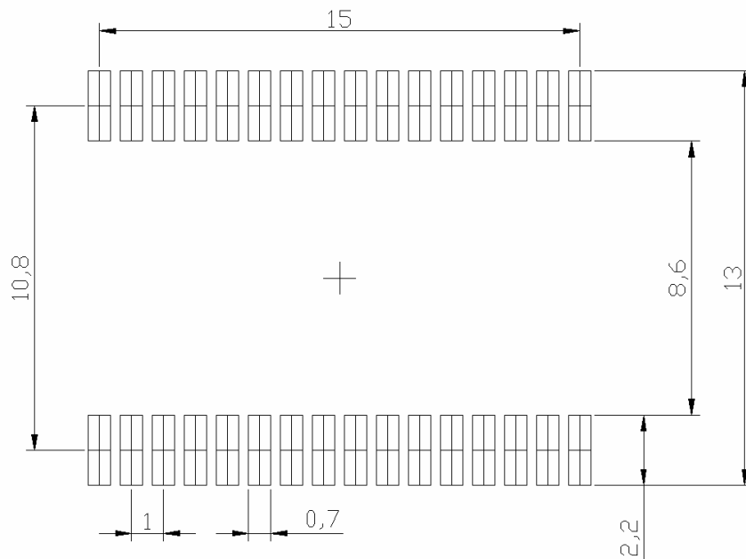
Figure 14. SCR1100 footprint.
