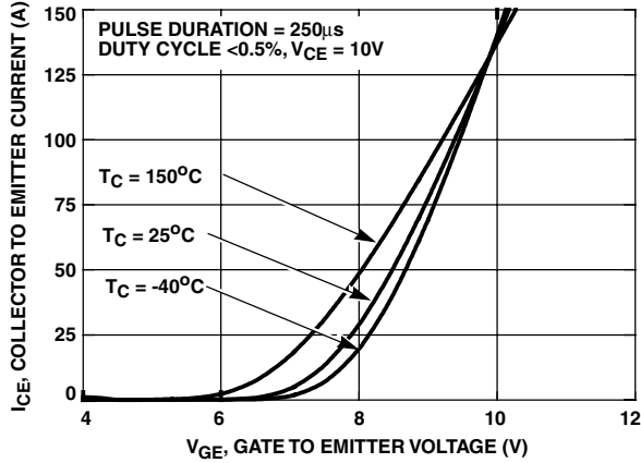
FIGURE 1. TRANSFER CHARACTERISTICS
