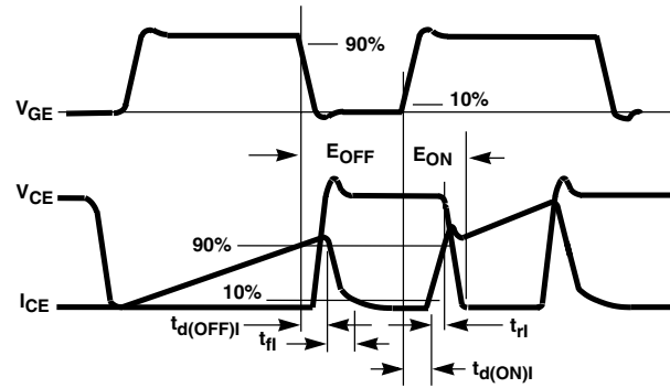
FIGURE 19. SWITCHING TEST WAVEFORMS
