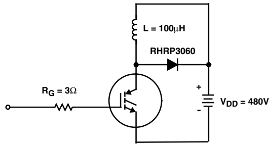
FIGURE 18. INDUCTIVE SWITCHING TEST CIRCUIT
