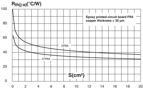
Figure 10. Thermal resistance junction to ambient versus copper surface under tab (DPAK and D²PAK)
