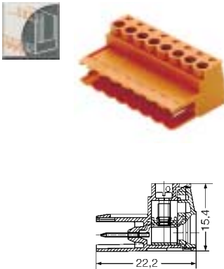
Pin plugs SLS 5.08/180
