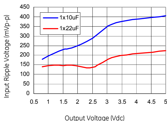
Figure 40. Input ripple voltage for various output voltages with 1x10 \mu F or 1x22 \mu F ceramic capacitors at the input (6A load). Input voltage is 12V.
