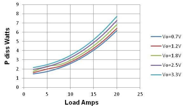
Figure 10 Power Dissipation Vin=12V, Fsw=500KHz
