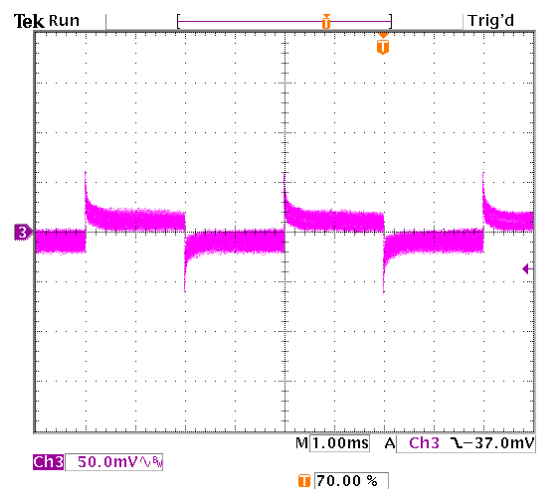
Figure 53. Transient Response with Regulation set to 0.74 mV/A
