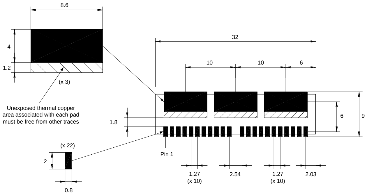
Figure 62. Recommended Pad Sizes
