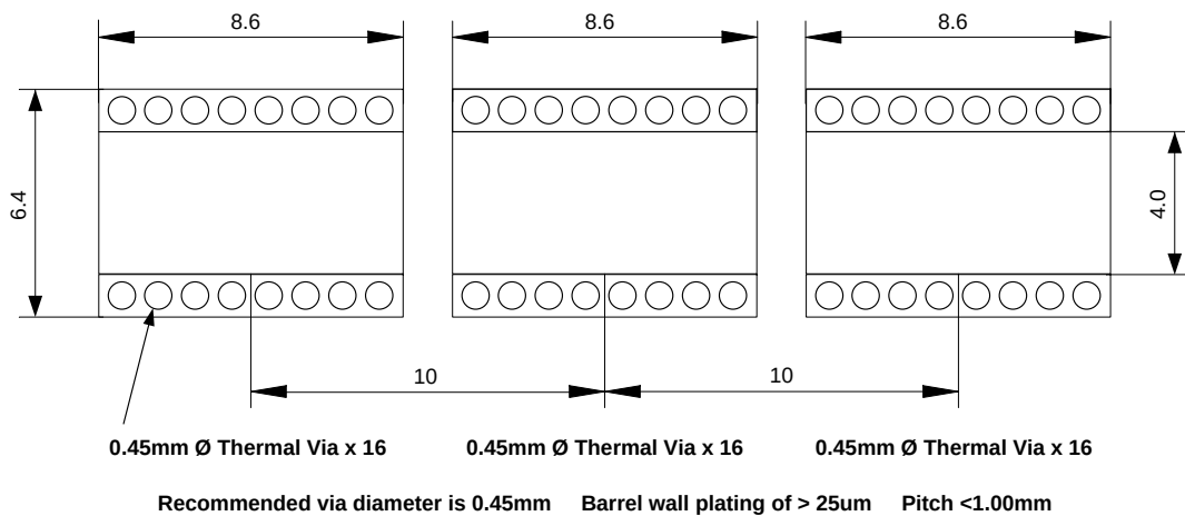
Figure 63. Recommended PCB Power Tab (Pins 23 - 25) Layout for Multilayer PCBs
