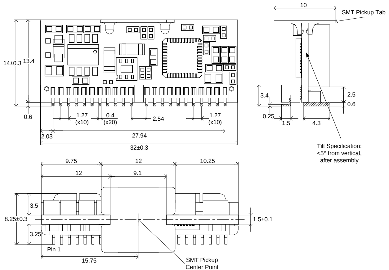
Figure 60. Mechanical Drawing
