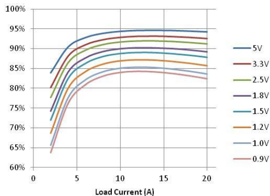
Figure 5. Efficiency vs. Load. V_{in}=12\text{V} , F_{sw}=500\text{KHz}
