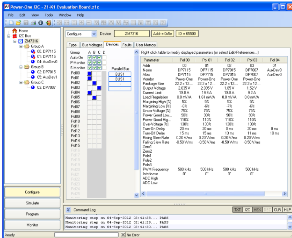
Figure 55 Evaluation Board Configuration showing Current Share Bus Assignment
