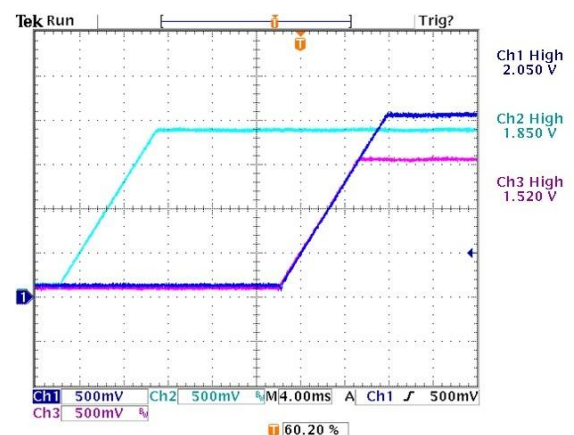
Figure 28 Two outputs delayed 5ms. All slew rates at 0.5V/ms.
