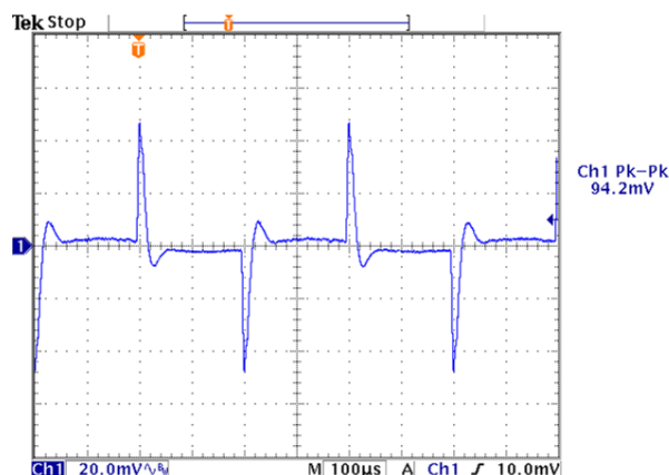
Figure 18 Transient Response with Regulation set to 0 mV/A.
