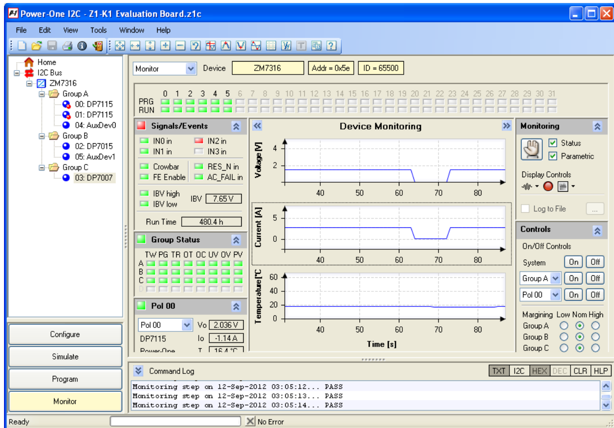
Figure 54. DPM Monitoring Window
