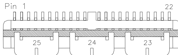
Figure 61. Pinout Diagram (Bottom View)
