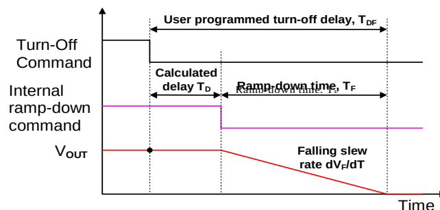
Figure 22. Relationship between Turn-Off Delay and Falling Slew Rate
