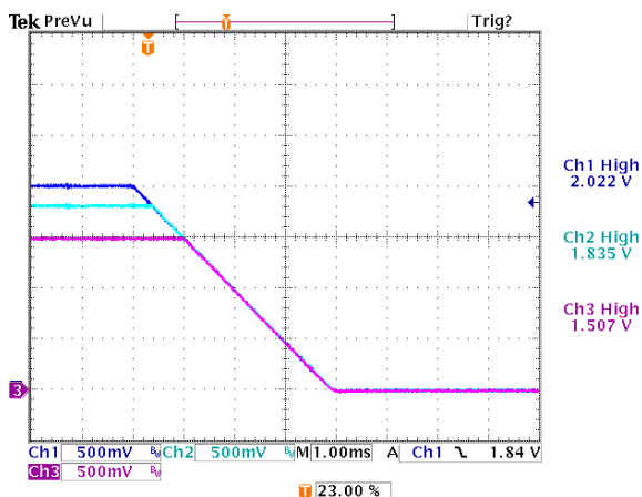
Figure 30. Tracking Turn-Off. Falling Slew Rate is Programmed at 0.5V/ms.
