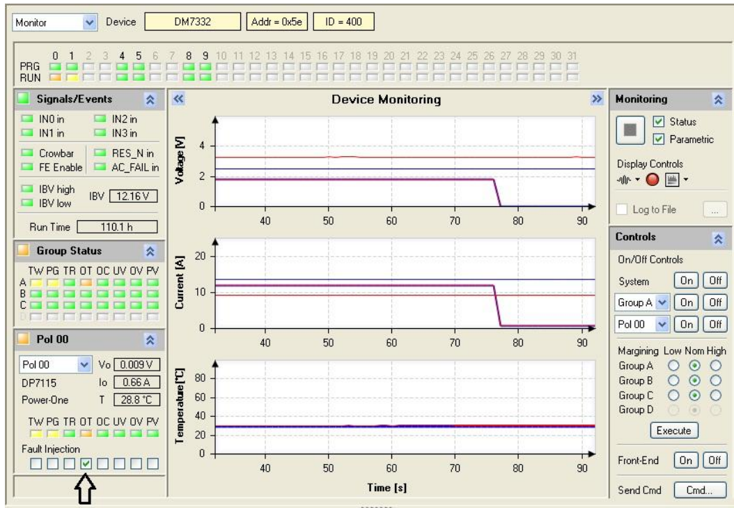
Figure 57. Example Overtemp Fault Injection in the GUI
