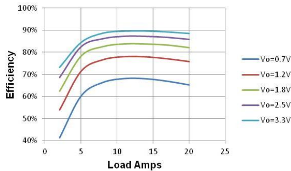
Figure 11 Efficiency vs Load, Vin=12V, Fsw=1MHz
