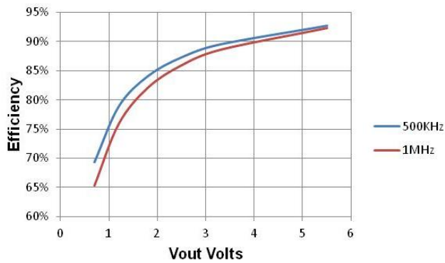
Figure 7 Efficiency vs Vout at Vin=12V, Load=20A
