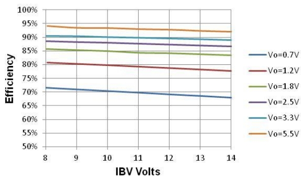
Figure 9 Efficiency vs Vin. Fsw=500kHz
