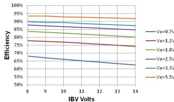
Figure 13 Efficiency vs Vin, Fsw=1MHz
