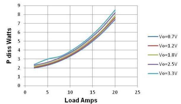
Figure 14 Dissipation vs Load. Vin=12V, Fsw=1MHz
