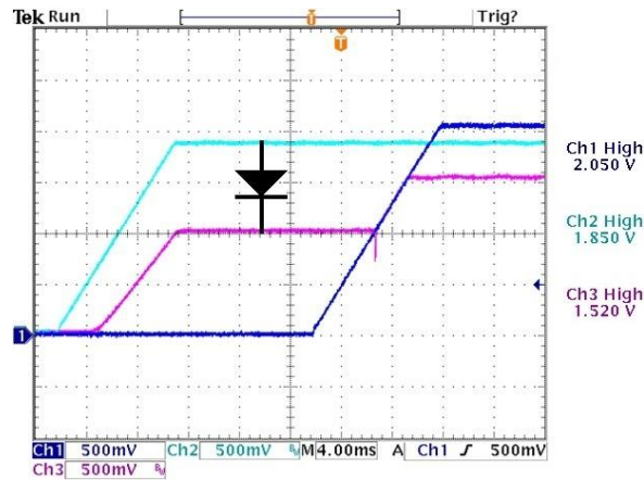
Figure 29. Turn On into Prebiased Load. V3 is Prebiased by V2 via a Diode.
