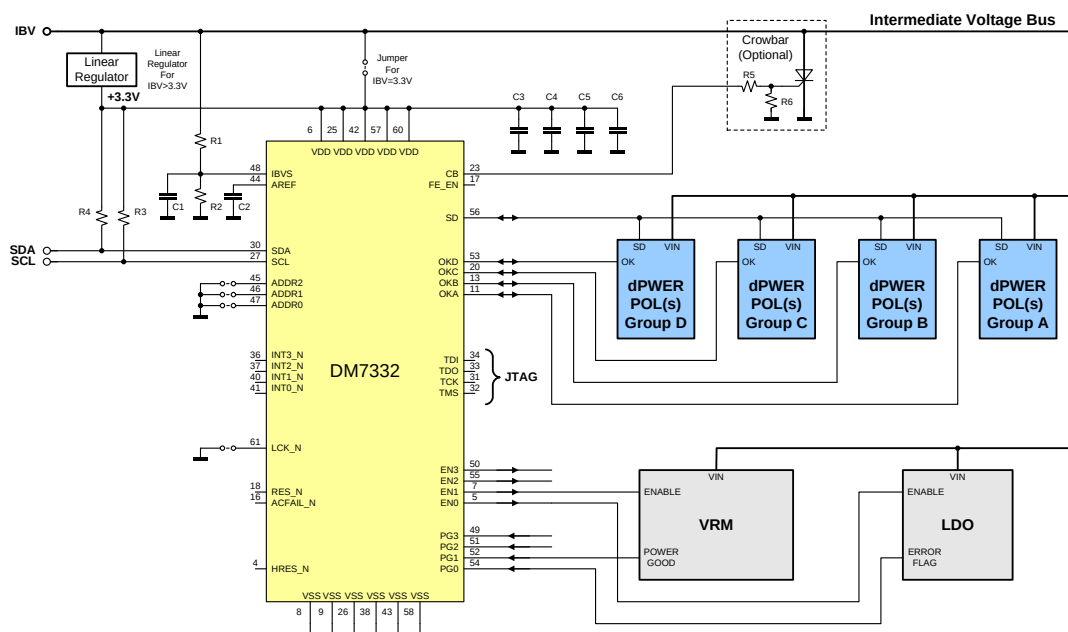
Figure 58. Multi-dPOL Power System Diagram
