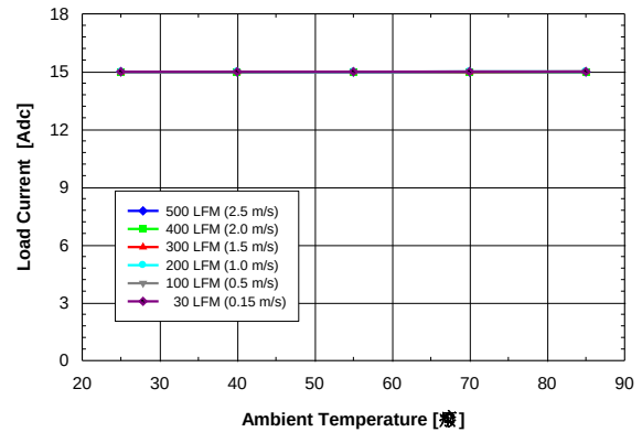
Figure 4. Available output current vs. ambient air temperature and airflow rates for converter DP7120G mounted horizontally with air flowing from input to output, MOSFET temperature \leq 120^{\circ}\text{C} , V_{in} = 12\text{ V} , V_{out} = 5\text{ V} , and F_{sw} = 1\text{MHz}
