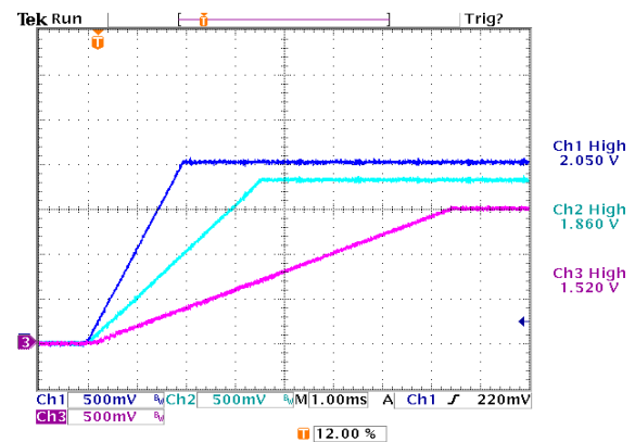
Figure 26. Turn-On with Different Rising Slew Rates. Rising Slew Rates are V1-1V/ms, V2-0.5V/ms, V3-0.2V/ms.
