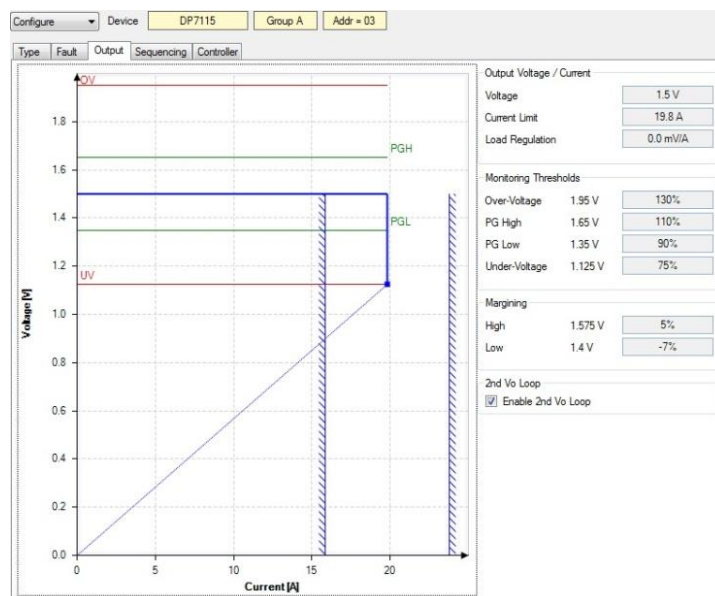
Figure 15. Output Configuration Window
