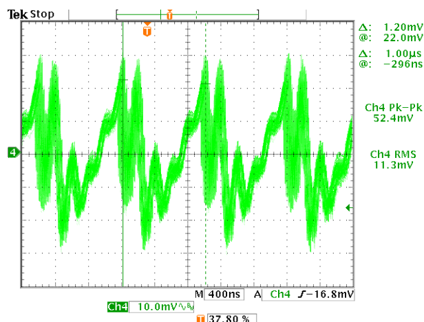
Figure 47. Input Voltage Noise, No Interleave
