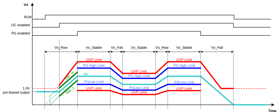
Figure 34. Protection Enable Conditions
