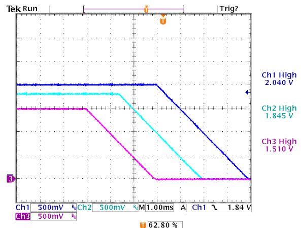
Figure 31. Turn-Off with Tracking and Sequencing. Falling Slew Rate is Programmed at 0.5V/ms.
