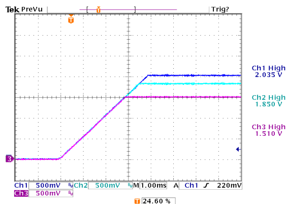
Figure 25. Tracking Turn-On. Rising Slew Rate is Programmed at 0.5V/ms for each output.
