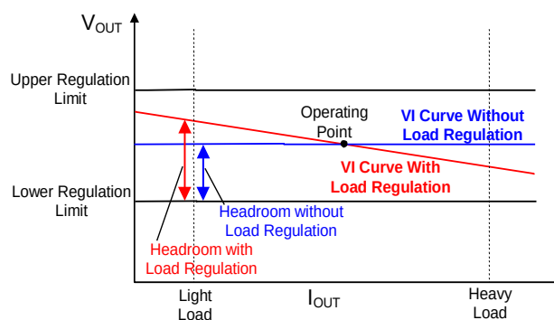
Figure 17. Optimal Voltage Positioning Concept
