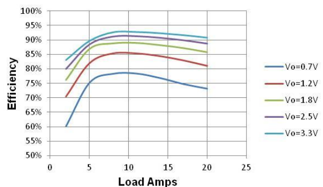
Figure 6 Efficiency vs. Load. V_{in}=8\text{V} , F_{sw}=500\text{KHz}
