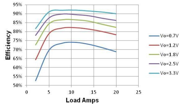
Figure 12 Efficiency vs Load, Vin=8V, Fsw=1MHz
