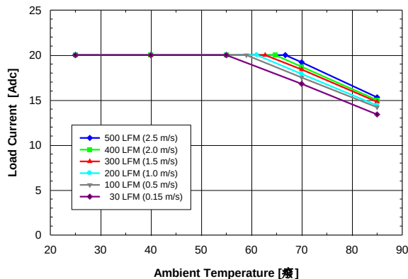
Figure 3. Available output current vs. ambient air temperature and airflow rates for converter DP7120G mounted horizontally with air flowing from input to output, MOSFET temperature \leq 120^{\circ}\text{C} , V_{in} = 12\text{ V} , V_{out} = 5\text{ V} , and F_{sw} = 500\text{KHz}
