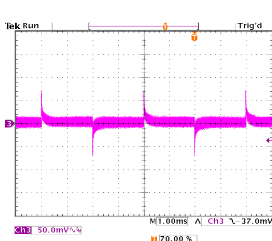
Figure 52. Transient Response with Regulation set to 0.0 mV/A.
