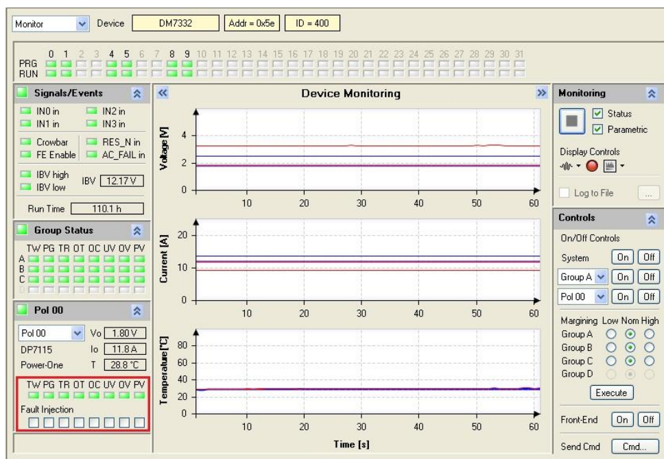
Figure 56. Fault Injection Controls In Monitor Window
