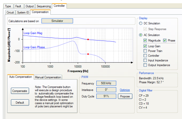
Figure 45. PWM Controller Window
