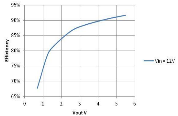
Figure 8 Efficiency vs. Output Voltage, Iout=7A, Fsw=500kHz
