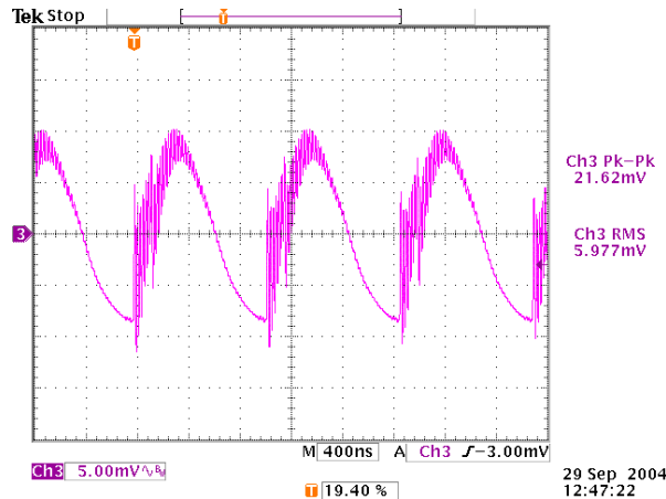
Figure 49. Output Voltage Noise, Full Load, No Interleave
