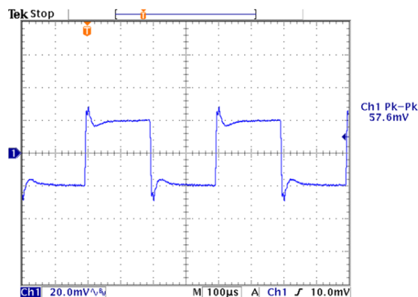
Figure 19 Transient response with Regulation set to 074 mV/A.
