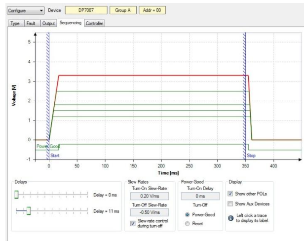
Figure 20. dPOL Configure Sequencing Window
