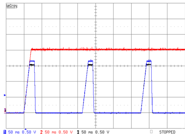
Figure 43. Turn-On into UVP on V3. The UV Fault Is Programmed To Be Non-Latching and Propagate From Group C to Group A. Ch1 – V3 (Group C), Ch2 – V2, Ch3 – V1 (Group A)
