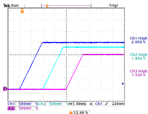
Figure 27. Sequenced Turn-On. Rising Slew Rate is Programmed at 1V/ms. V2 Delay is 2ms, V3 delay is 4ms.
