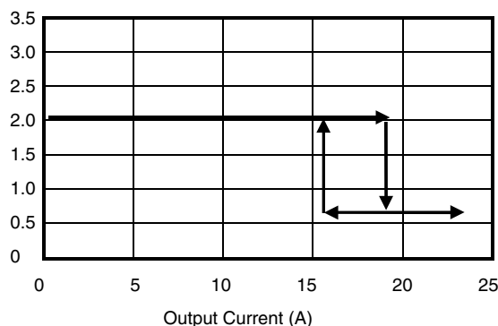
Figure 4. RC5052 Short Circuit Characteristic
