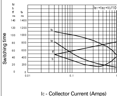
Switching Speeds
