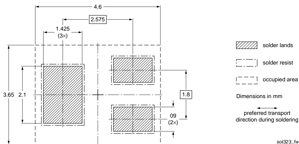
Fig 20. Wave soldering footprint for SOT323 (SC-70)
