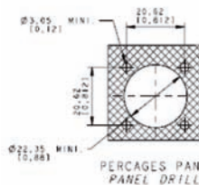
PERCAGES PANNEAU PANEL DRILLING
