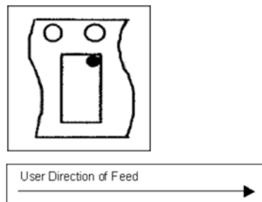
Figure 29. LGA-14 package orientation in carrier tape
