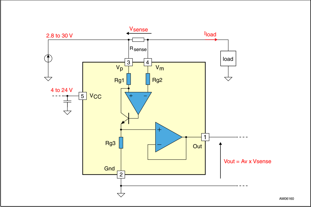
Figure 1. Application schematics
