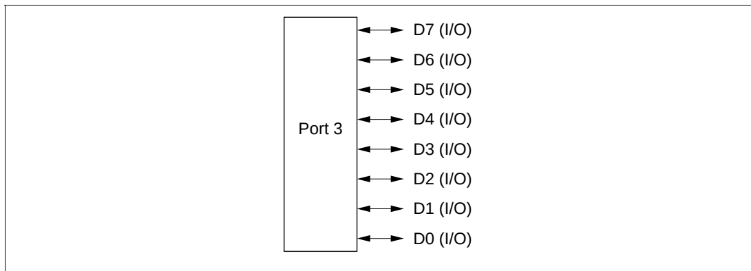
Figure 8.10 Port 3 Pin Functions (Modes 1, 2, and 3 (EXPE = 1))
